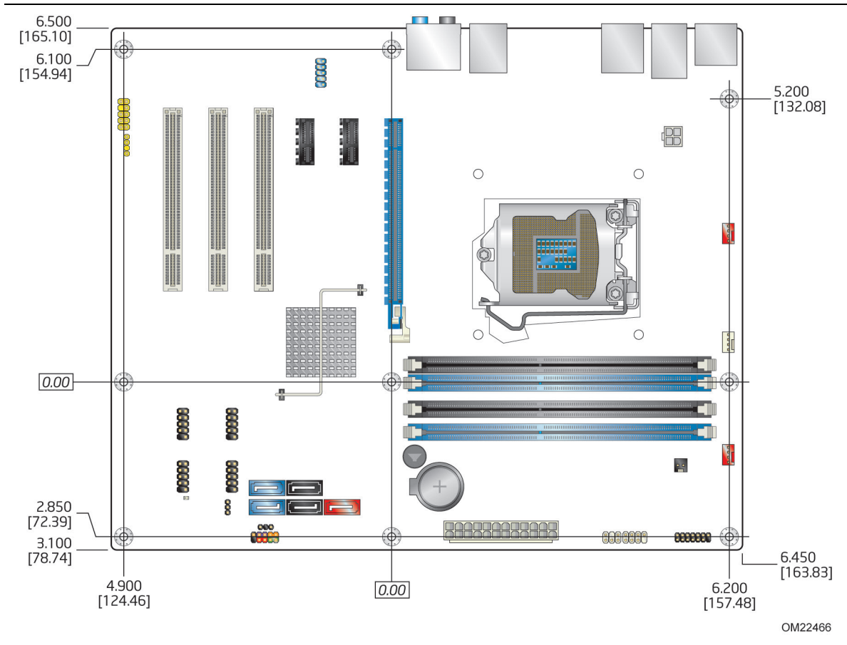
Figure 14. Board Dimensions
