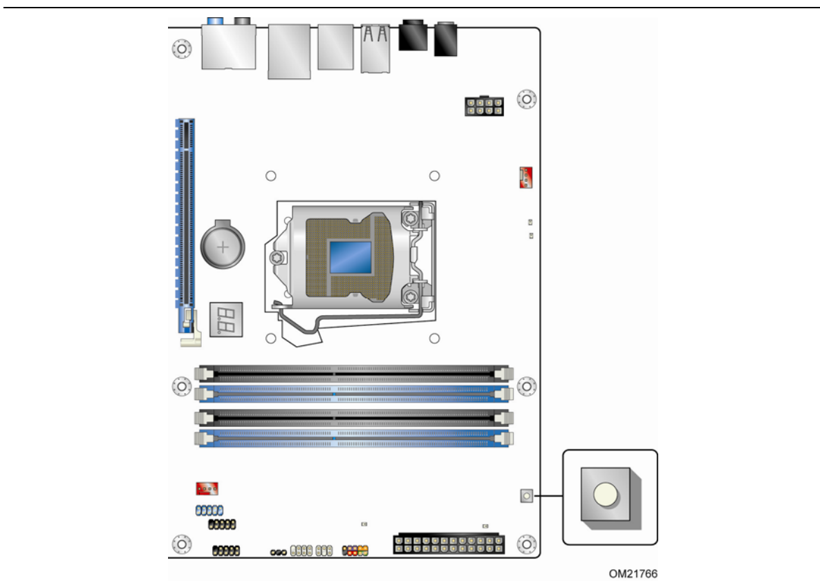
Figure 8. Location of the Onboard Power Button
