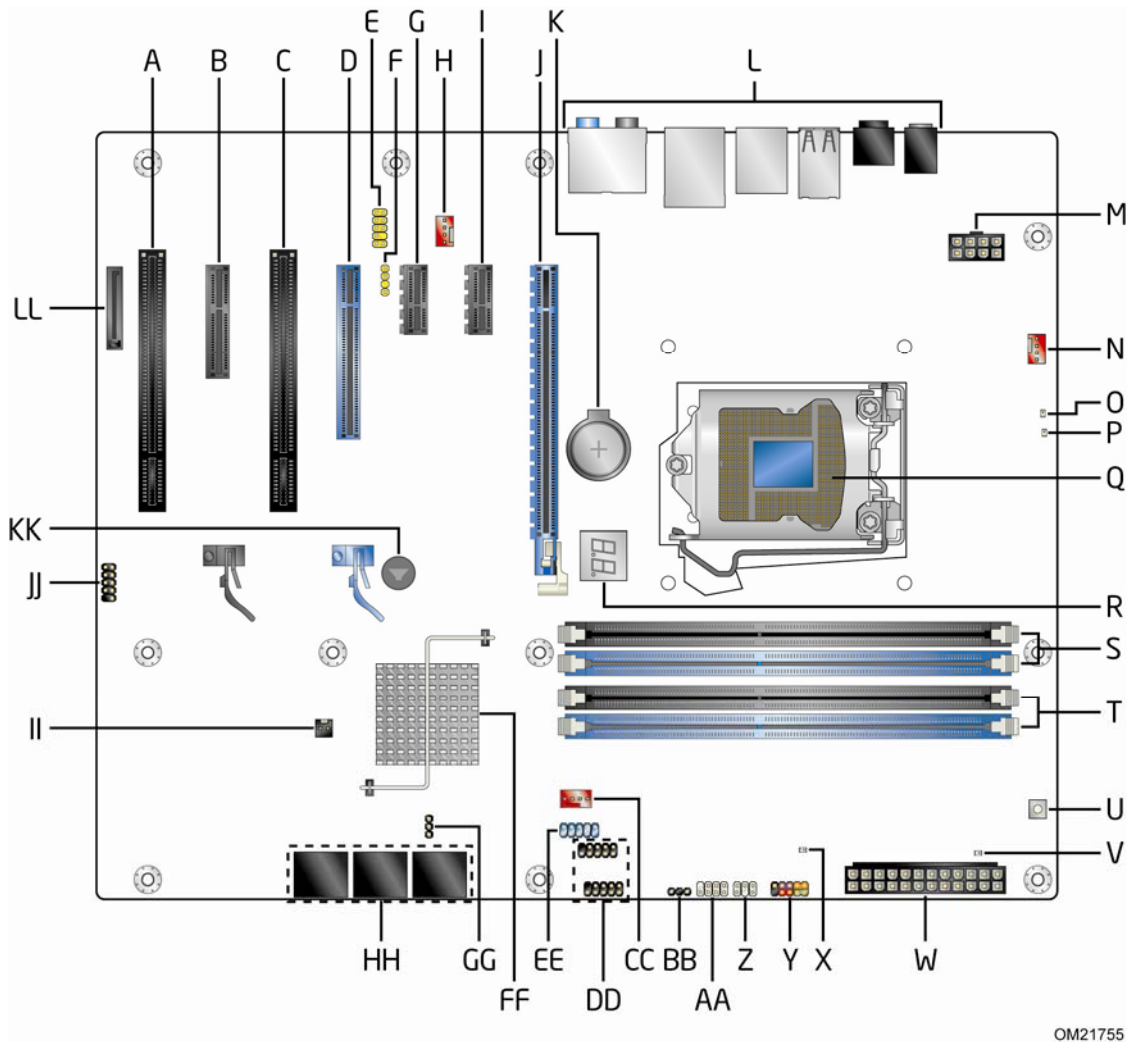
Figure 1. Major Board Components
