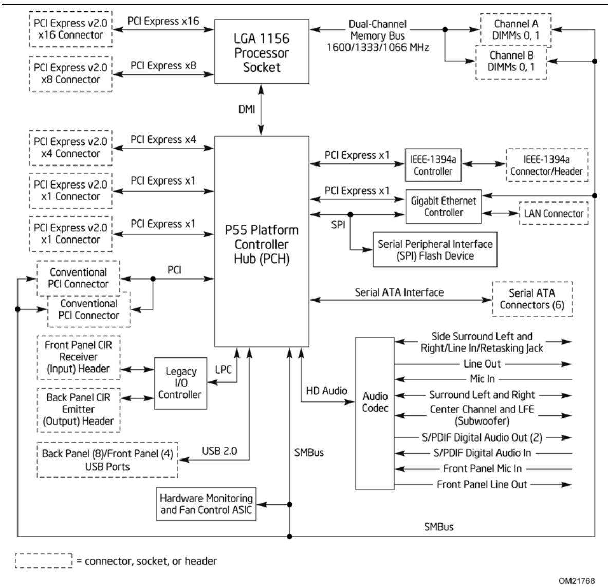
Figure 2. Block Diagram
