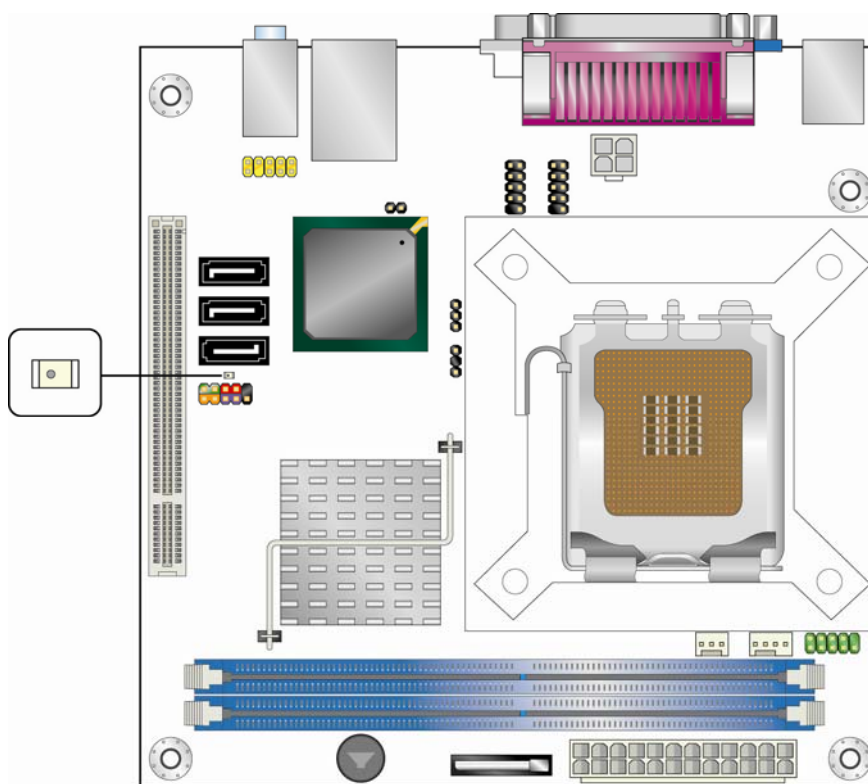
Figure 7. Location of the Standby Power Indicator LED
