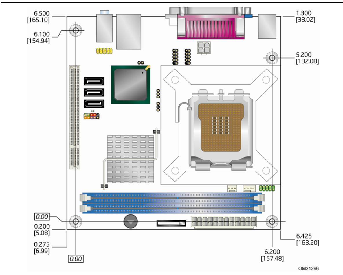
Figure 14. Board Dimensions
