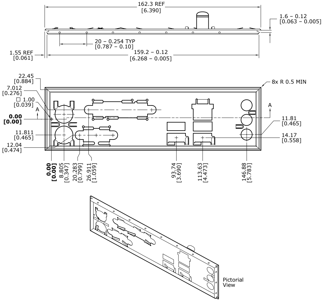
Figure 27. I/O Shield Dimensions for Boards with the 6-Channel (5.1) Audio Subsystem
