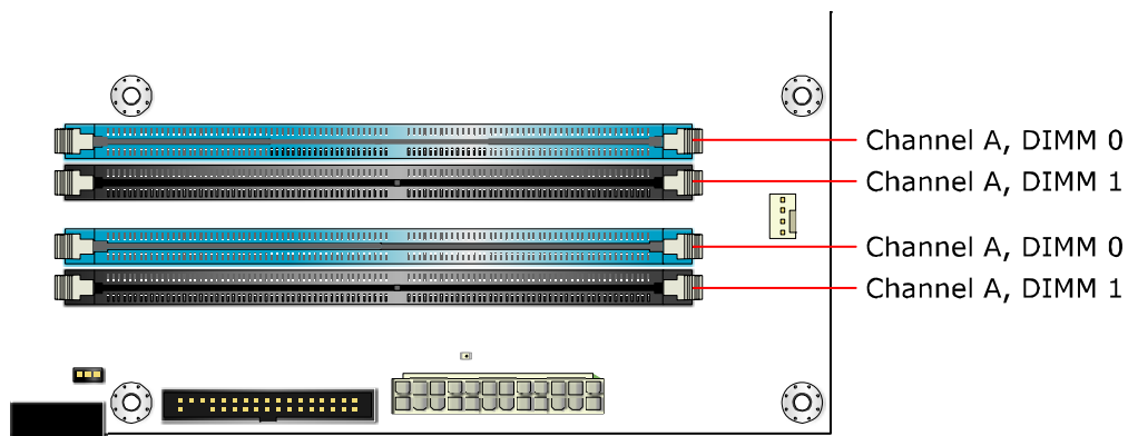
Figure 3. Memory Channel and DIMM Configuration
