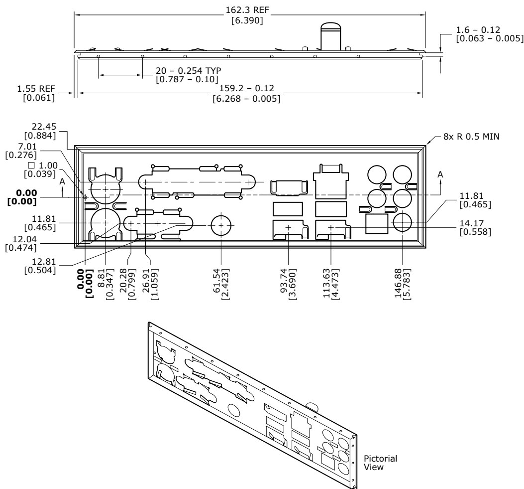
Figure 26. I/O Shield Dimensions for Boards with the 8-Channel (7.1) Audio Subsystem
