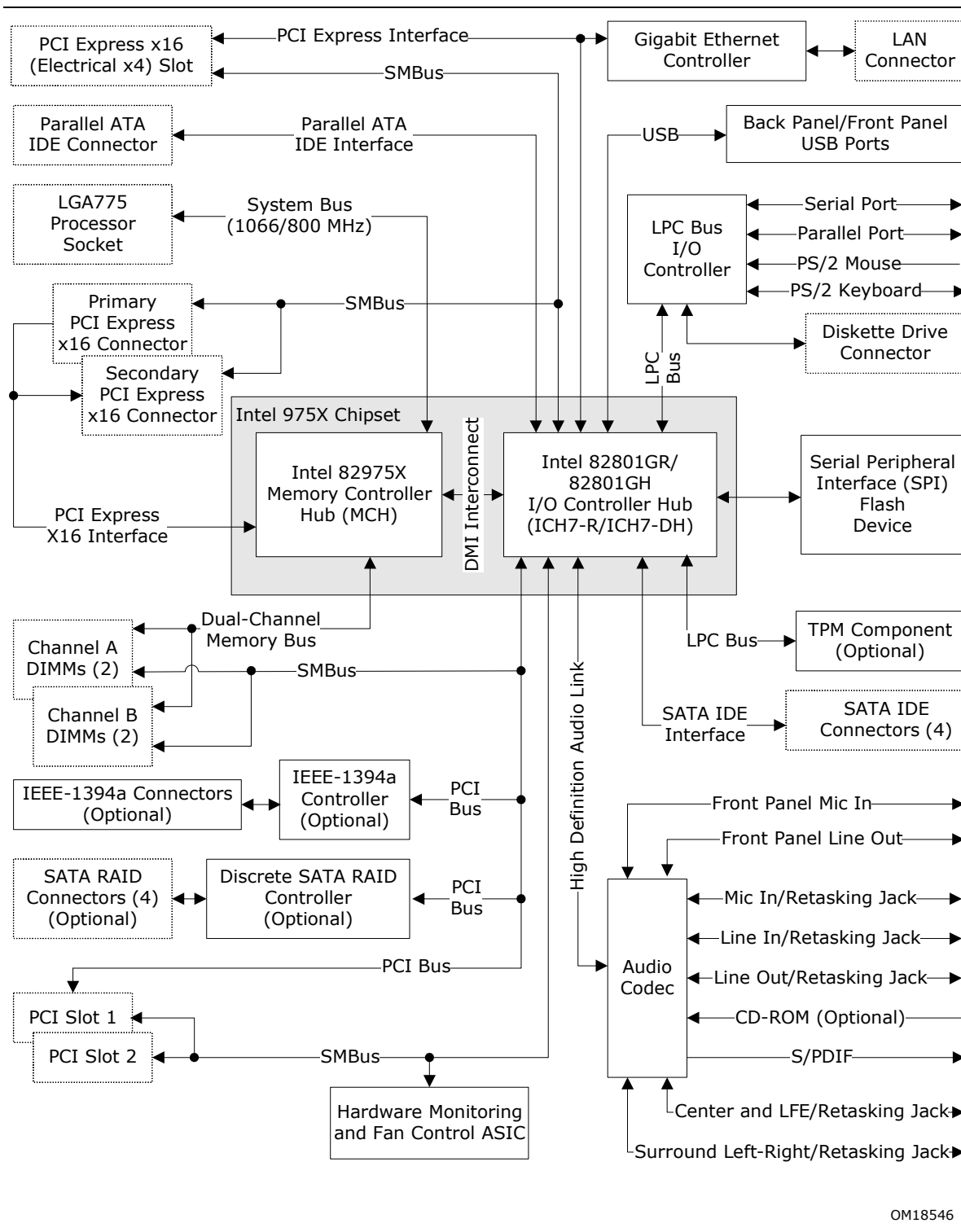
Figure 2. Block Diagram
