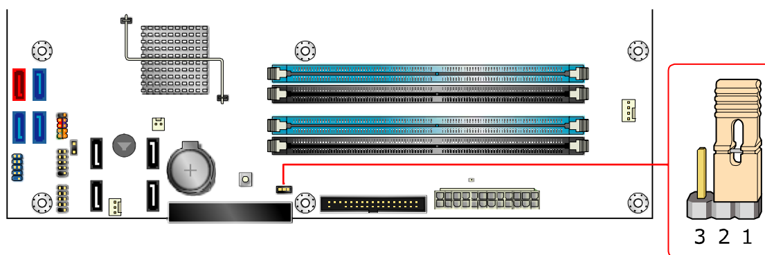
Figure 24. Location of the Jumper Block
