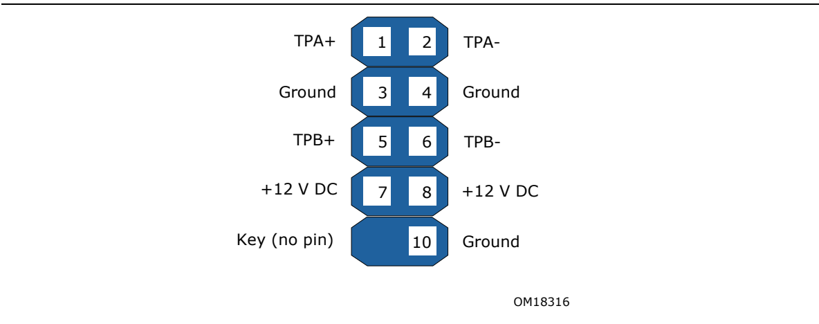
Figure 23. Connection Diagram for Front Panel IEEE 1394a Header
