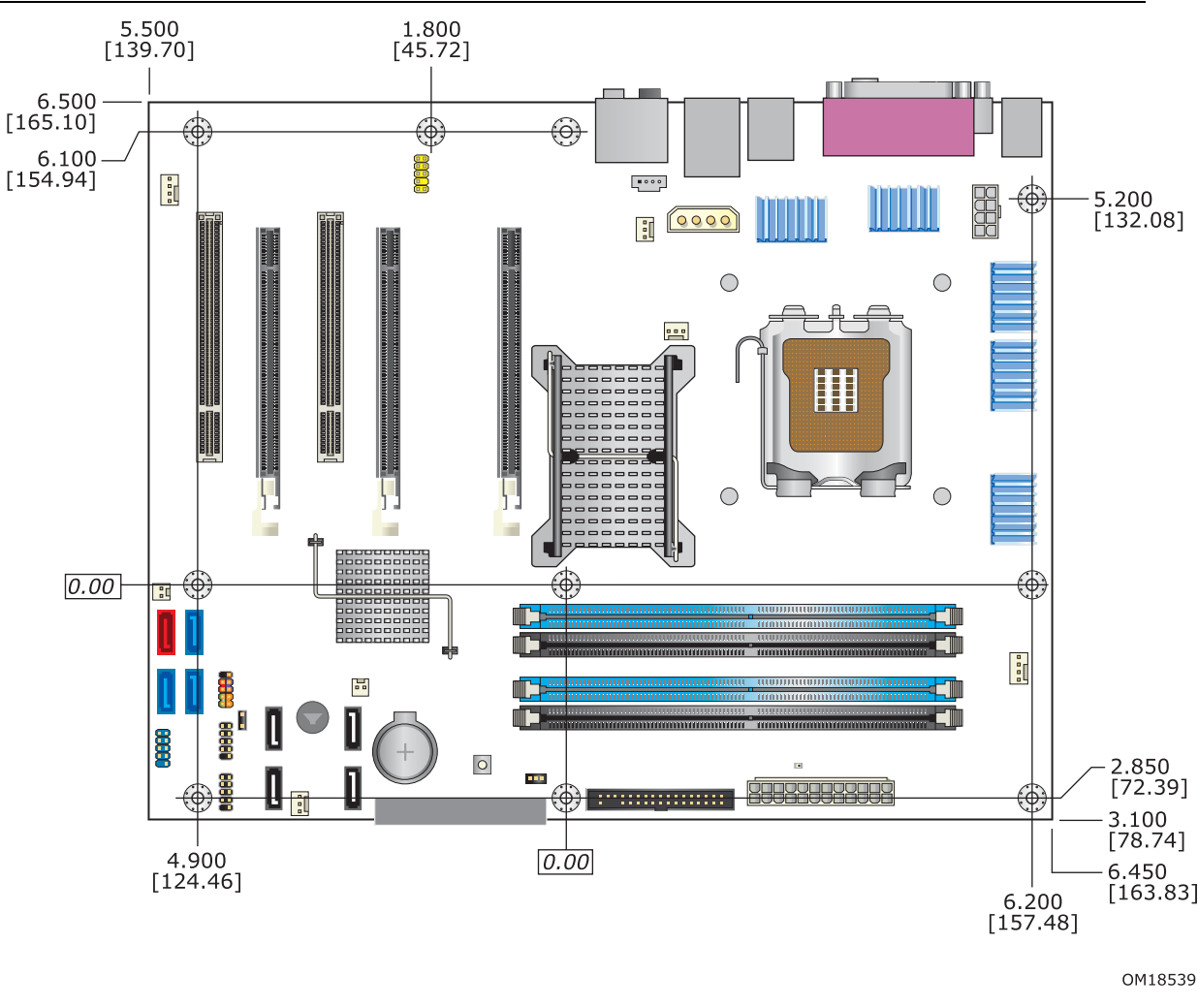
Figure 25. Board Dimensions
