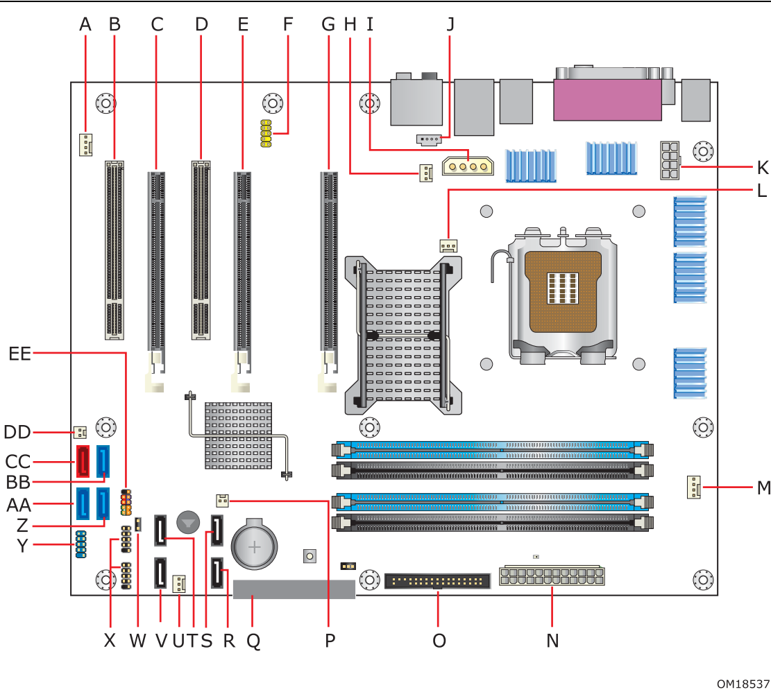
Figure 20. Component-side Connectors and Headers
