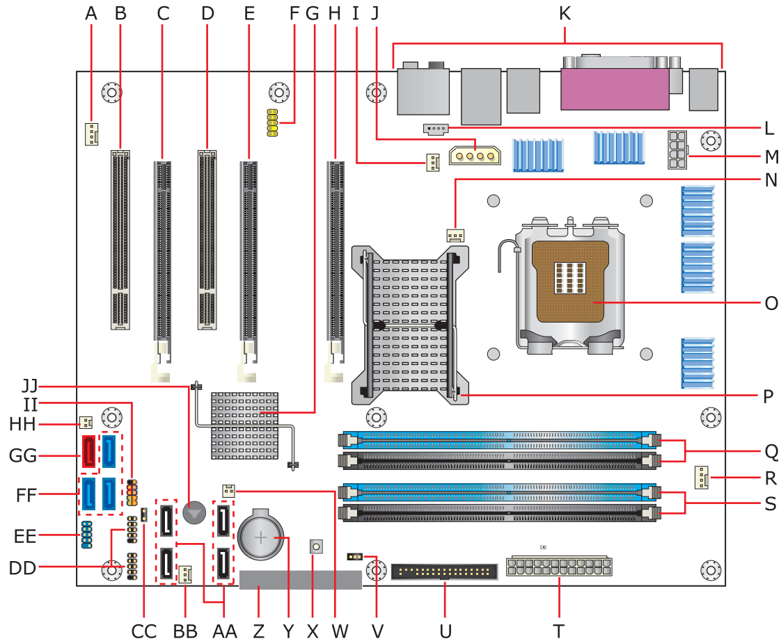
Figure 1. Desktop Board Components
