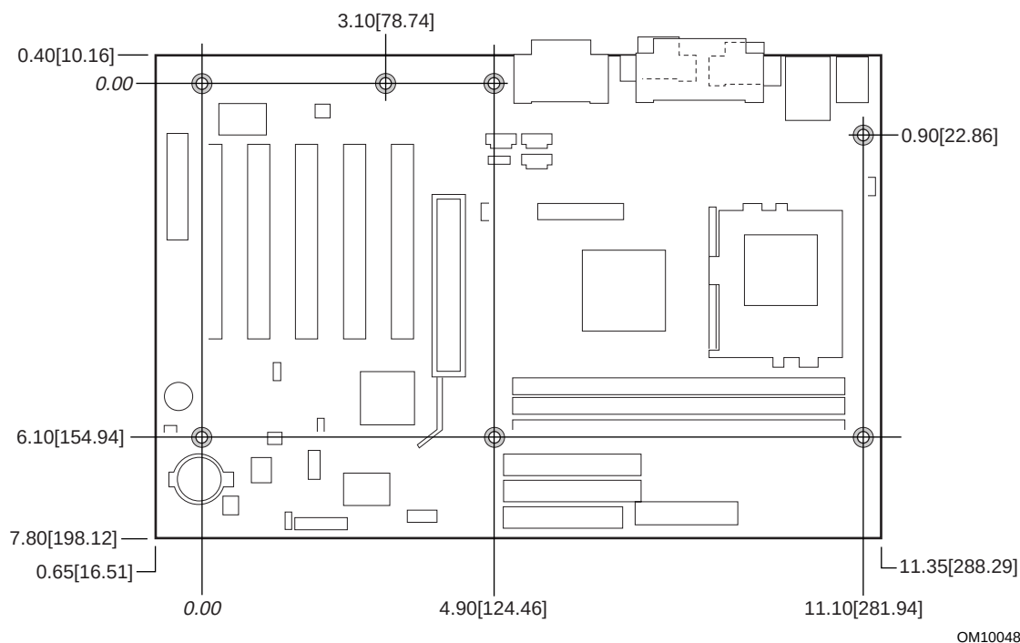
Figure 14. D815EEA Board Dimensions
