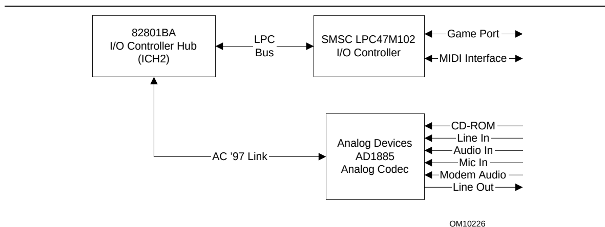
Figure 4. Block Diagram of Basic Audio Subsystem
