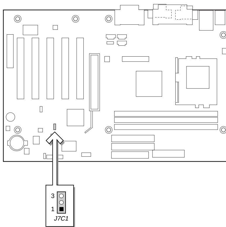
Figure 13. Location of the Jumper Block
