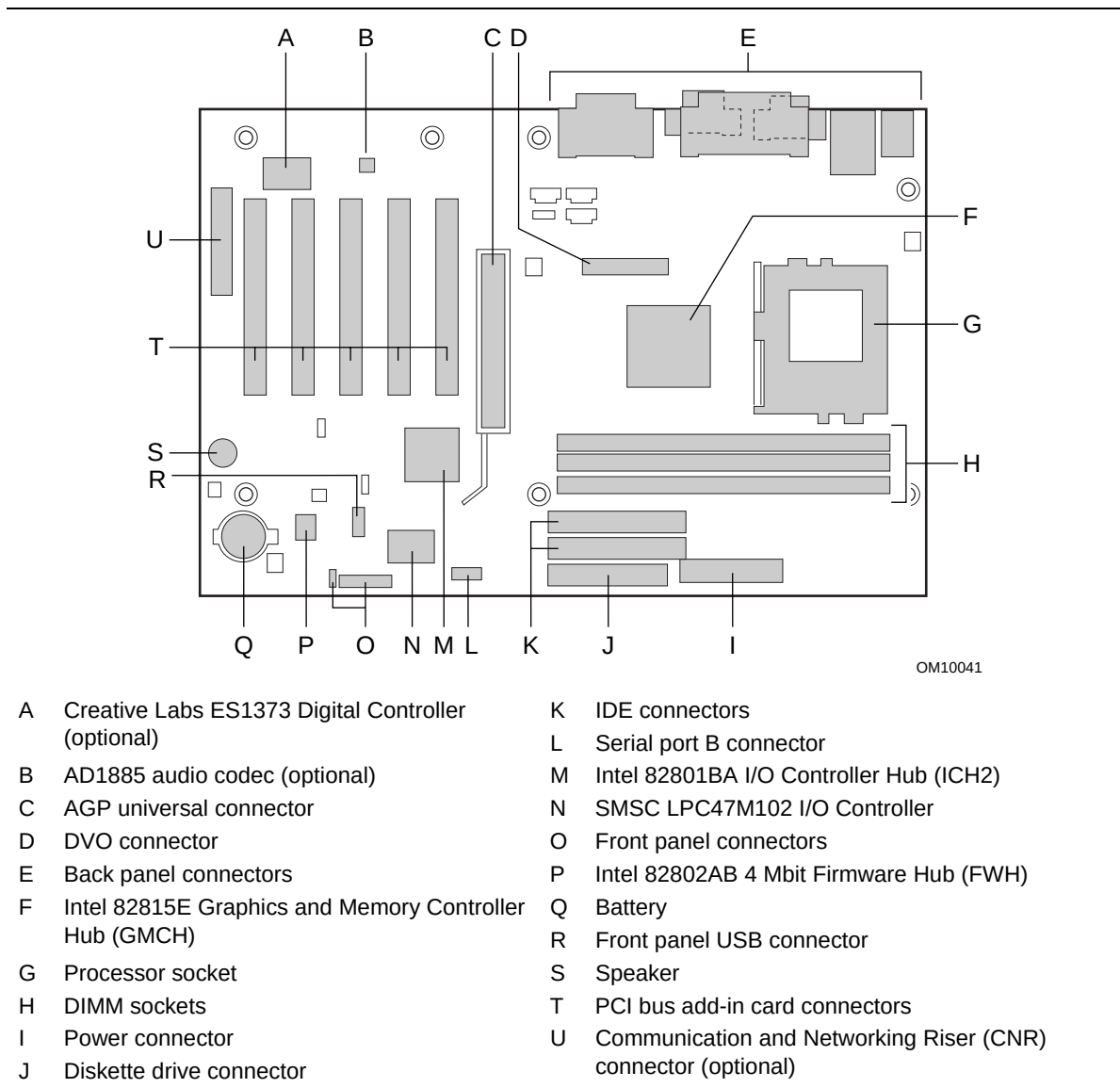
Figure 1. D815EEA Board Components
