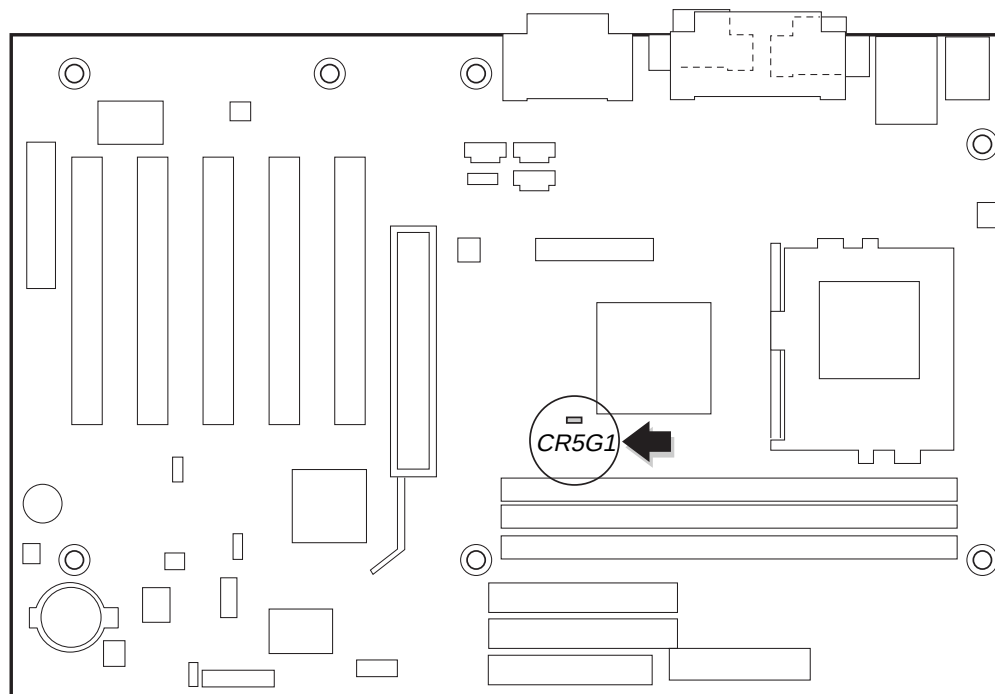
Figure 8. Location of Standby Power Indicator LED
