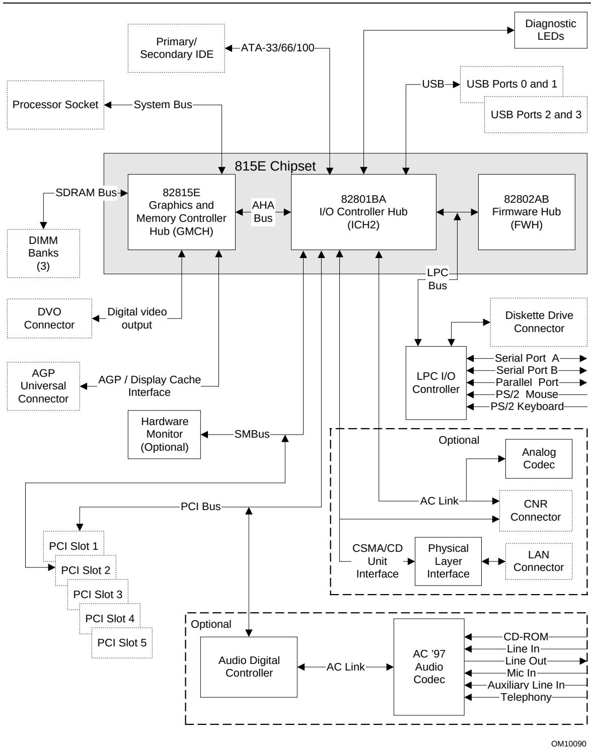
Figure 2. Block Diagram
