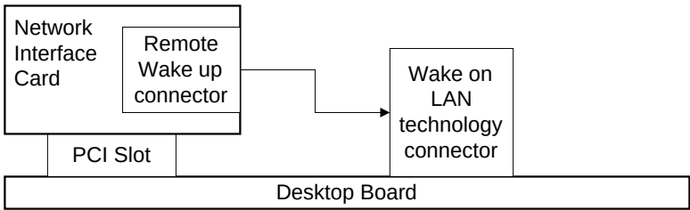
Figure 7. Using the Wake on LAN Technology Connector
