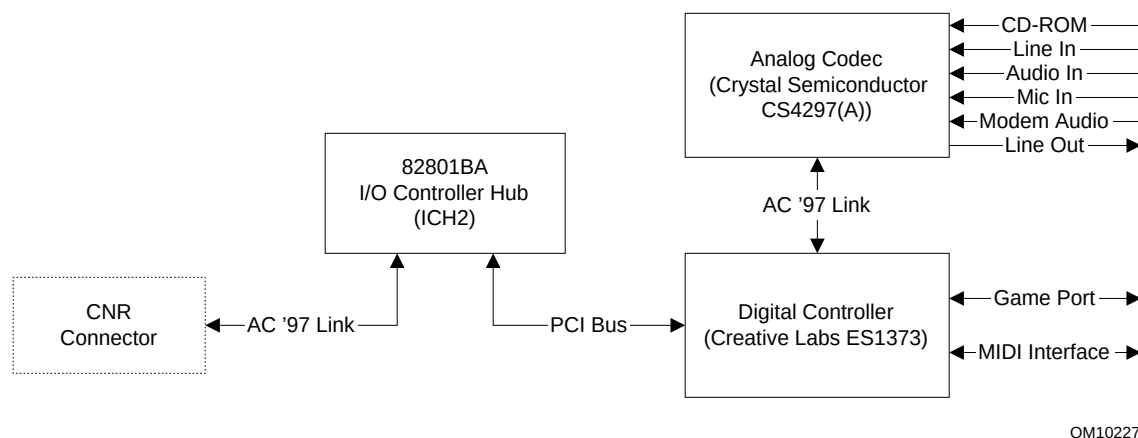
Figure 5. Block Diagram of Enhanced PCI Audio Subsystem
